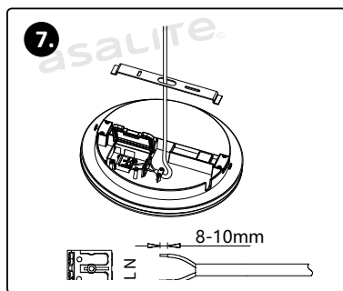
Open the junction box. Connect the wires. Cover the junction box, lock the screws!
