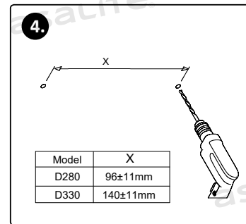
Drill holes according to the installation position!
